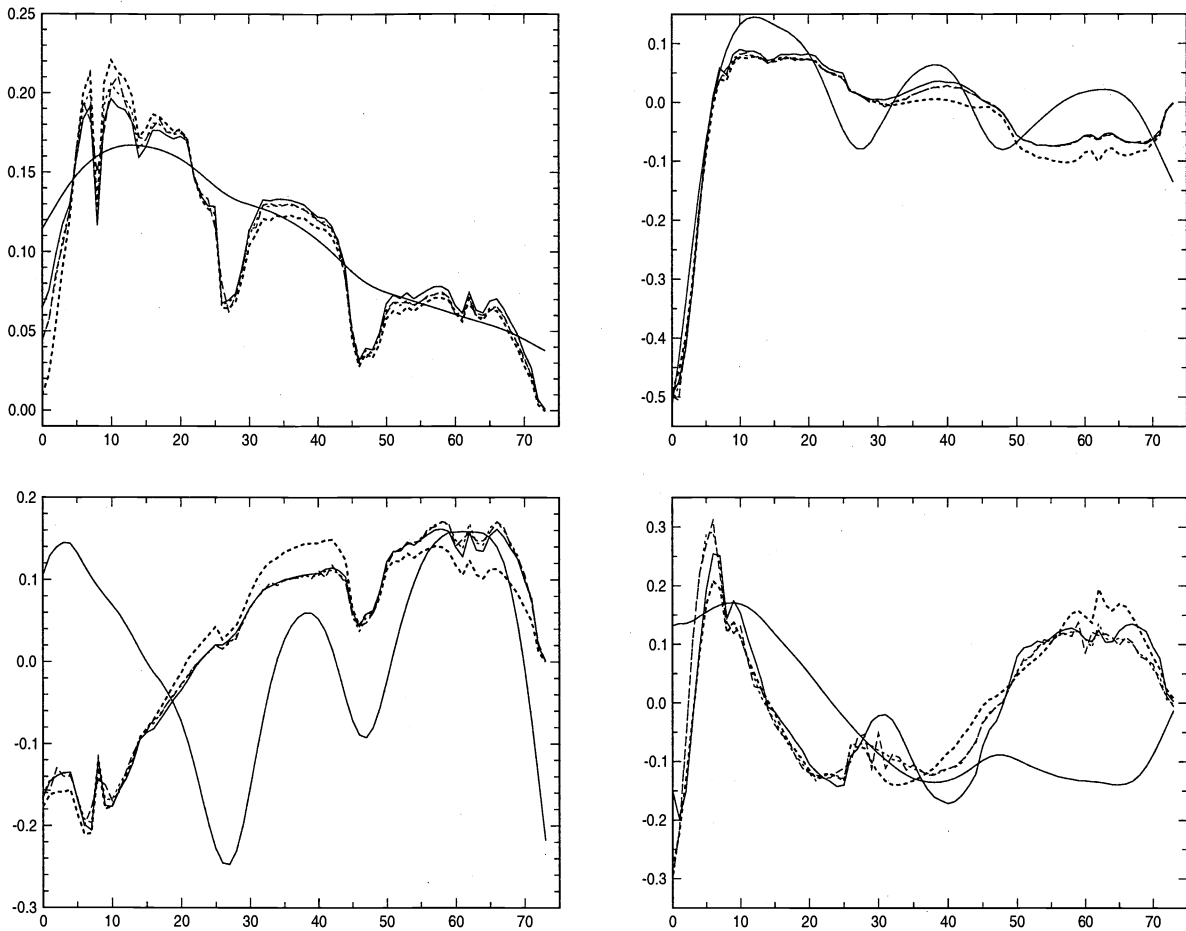
Figure 3: Chromatic eigenvectors of subsets of spatial Fourier transforms of the original data and the pseudo inverse: solid line : disk of the original data, solid line : disk of the pseudo inverse, dotted line : 60-80 annulus of the original data, dashed line : 60-80 annulus of the pseudo inverse, heavy dotted line : "threshold = 2" mask of the pseudo inverse. The eigenvector plots are ordered left to right and top to bottom.
