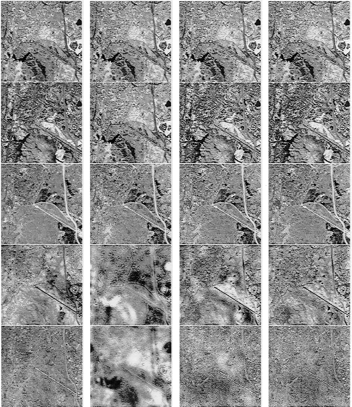
Figure 5: The first five (top to bottom) eigenimages of 'Jasper Ridge': the original AVIRIS sequence (first column), the pseudo-inverse (second column), the reconstruction with 1 principal component (third column), and the reconstruction with 3 principal components (fourth column). The reconstruction algorithm used threshold 2 and annulus 60-80.
